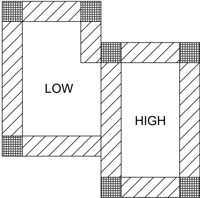
ROOF HEIGHT DIFFERENTIAL GREATER THAN 3' (90 cm)
